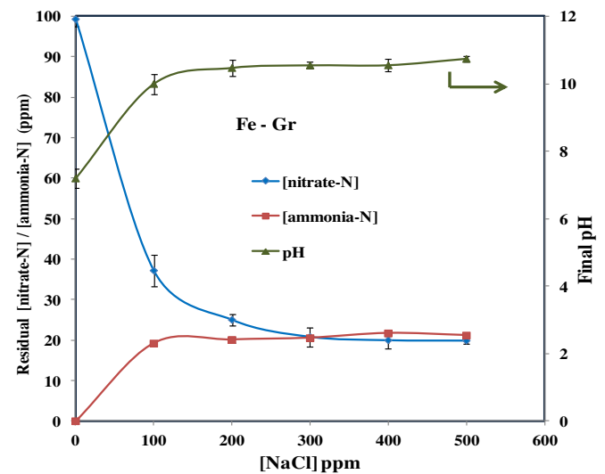
Fig. 4. Effect of NaCl concentration on nitrate removal by electrochemical method using Fe anode-Gr cathode. (Initial [nitrate-N] = 100 ppm, pH = 7, current density = 25 \text{ mA cm}^{-2} and electrolysis time = 180 min). Error bars are the standard deviations of triplicate experiments.
