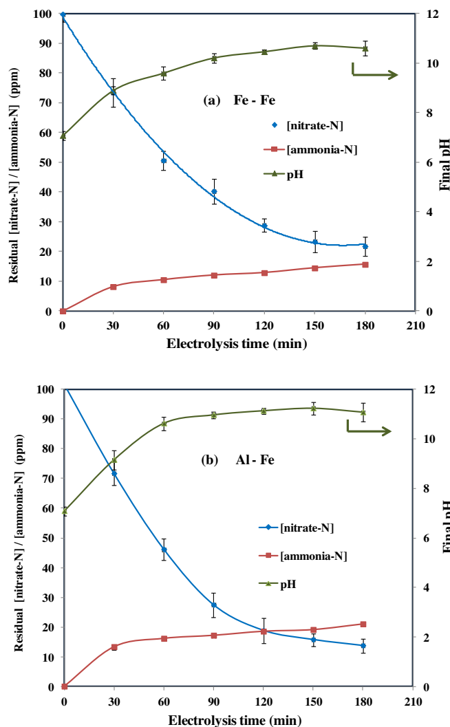
Fig. 3. Effect of electrolysis time on nitrate removal by electrochemical method using (a) Fe anode-Fe cathode and (b) Al anode -Fe cathode. (Initial [nitrate-N] = 100 ppm, [NaCl] = 100 ppm, pH=7 and current density = 25 mA cm -2 ). Error bars are the standard deviations of triplicate experiments.
